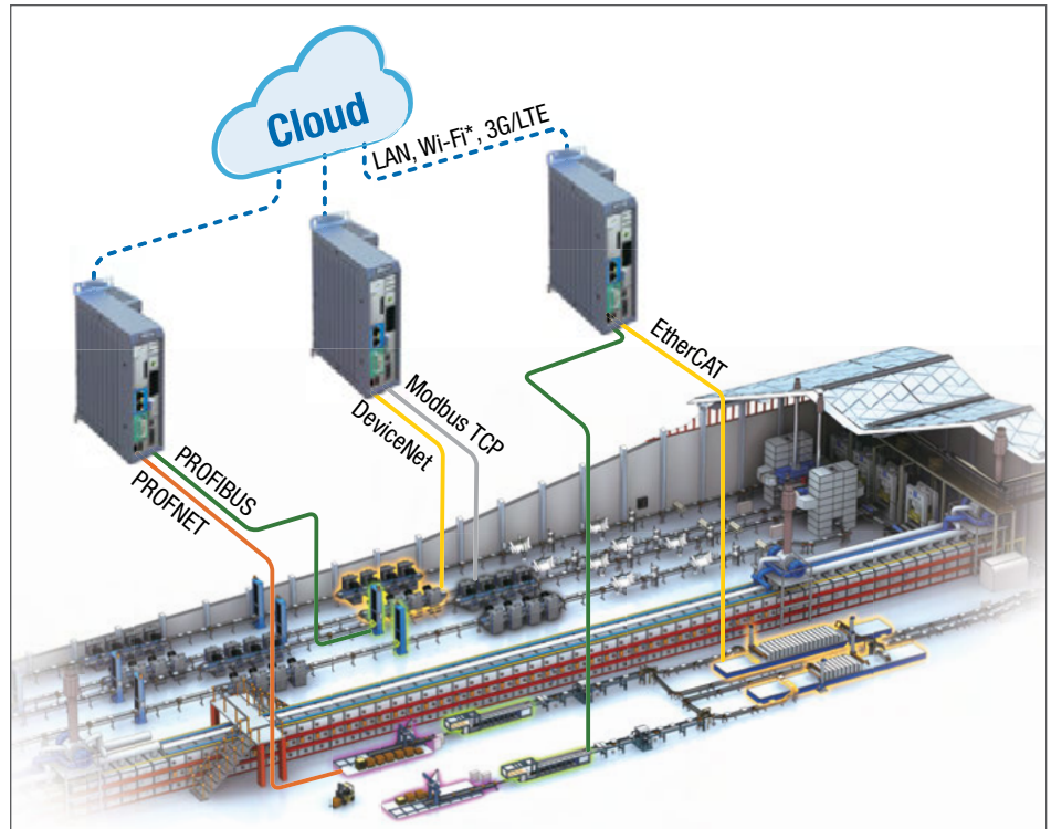
Figure 2. The NIFE 100 connects factory systems to the cloud.
